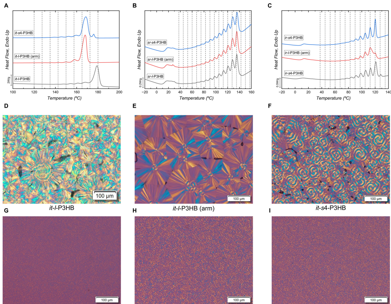
Fig. 2 Final DSC heating scans after SSA thermal fractionation (A–C) and PLOM micrographs (D–I) of it -P3HB ( it -s4-P3HB, it -P3HB, and it -l-P3HB (arm)) and sr -P3HB ( sr -s4-P3HB, sr -l-P3HB, and sr -l-P3HB (arm)). The (arm) denotes the lower molar mass linear P3HB with a chain length equivalent to one arm of star-shaped P3HB.
