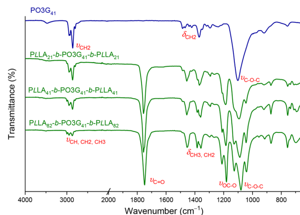
Fig. 4 FT-IR spectra of the \text{PO3G}_{41} macroinitiator and \text{PLLA}_m\text{-b-PO3G}_{41}\text{-b-PLLA}_m triblock copolymers.
