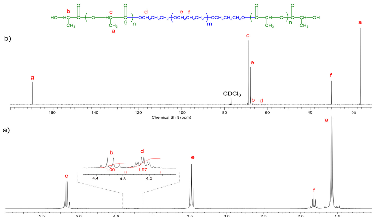
Fig. 3 (a) ^1\text{H} - and (b) ^{13}\text{C} -NMR spectra in \text{CDCl}_3 of the \text{PLLA}_{82}\text{-b-PO3G}_{41}\text{-PLLA}_{82} copolymer.
