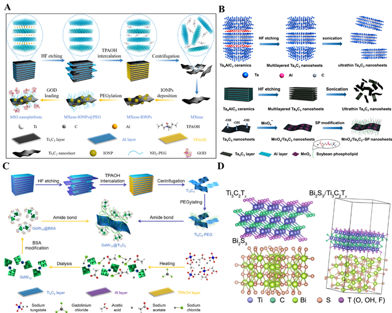
Fig. 3 Strategies for functionalizing MXenes with bioactive nanoparticles. (A) Schematic illustration of the successive synthetic procedures of 2D \text{Ti}_3\text{C}_2 MXene and MIG nanoplateforms for in vivo synergistic photothermal-enhanced nanocatalytic cancer therapy. 75 Reproduced from ref. 75 with permission from American Chemical Society, copyright 2019. (B) The scheme of the synthetic procedure for \text{Ta}_4\text{C}_3 and \text{MnO}_x/\text{Ta}_4\text{C}_3 -SP composite nanosheets, including HF etching, sonication exfoliation, in situ redox reaction between \text{Ta}_4\text{C}_3 nanosheets and postintroduced \text{KMnO}_4 , and subsequent surface SP modification. 78 Reproduced from ref. 78 with permission from American Chemical Society, copyright 2017. (C) Schematic illustration for the synthesis of \text{GdW}_{10}@\text{Ti}_3\text{C}_2 composite nanosheets, including chemical exfoliation of MAX-phase \text{Ti}_3\text{AlC}_2 ceramic to produce \text{Ti}_3\text{C}_2 MXene and further surface functionalization with \text{GdW}_{10} POM nanoclusters. 85 Reproduced from ref. 85 with permission from Tsinghua University Press, copyright 2018. (D) Crystal structure of \text{Ti}_3\text{C}_2\text{T}_x , \text{Bi}_2\text{S}_3 and \text{Ti}_3\text{C}_2\text{T}_x/\text{Bi}_2\text{S}_3 after structure optimization. 86 Reproduced from ref. 86 with permission from Springer Nature, copyright 2021.
