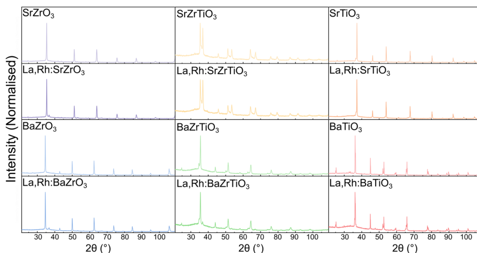
Fig. 2 X-ray diffraction patterns of base \text{ABO}_3 and \text{La,Rh:ABO}_3 perovskites.
