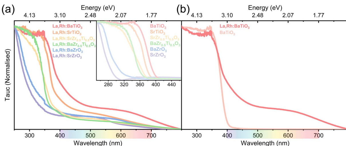
Fig. 3 (a) Normalised Tauc plot of \text{La,Rh:ABO}_3 perovskites. The inset contains Tauc plots for the base perovskites. (b) The Tauc of \text{La,Rh} co-doped and undoped BTO are plotted to demonstrate the visible light absorption conferred by \text{La,Rh} co-doping.
