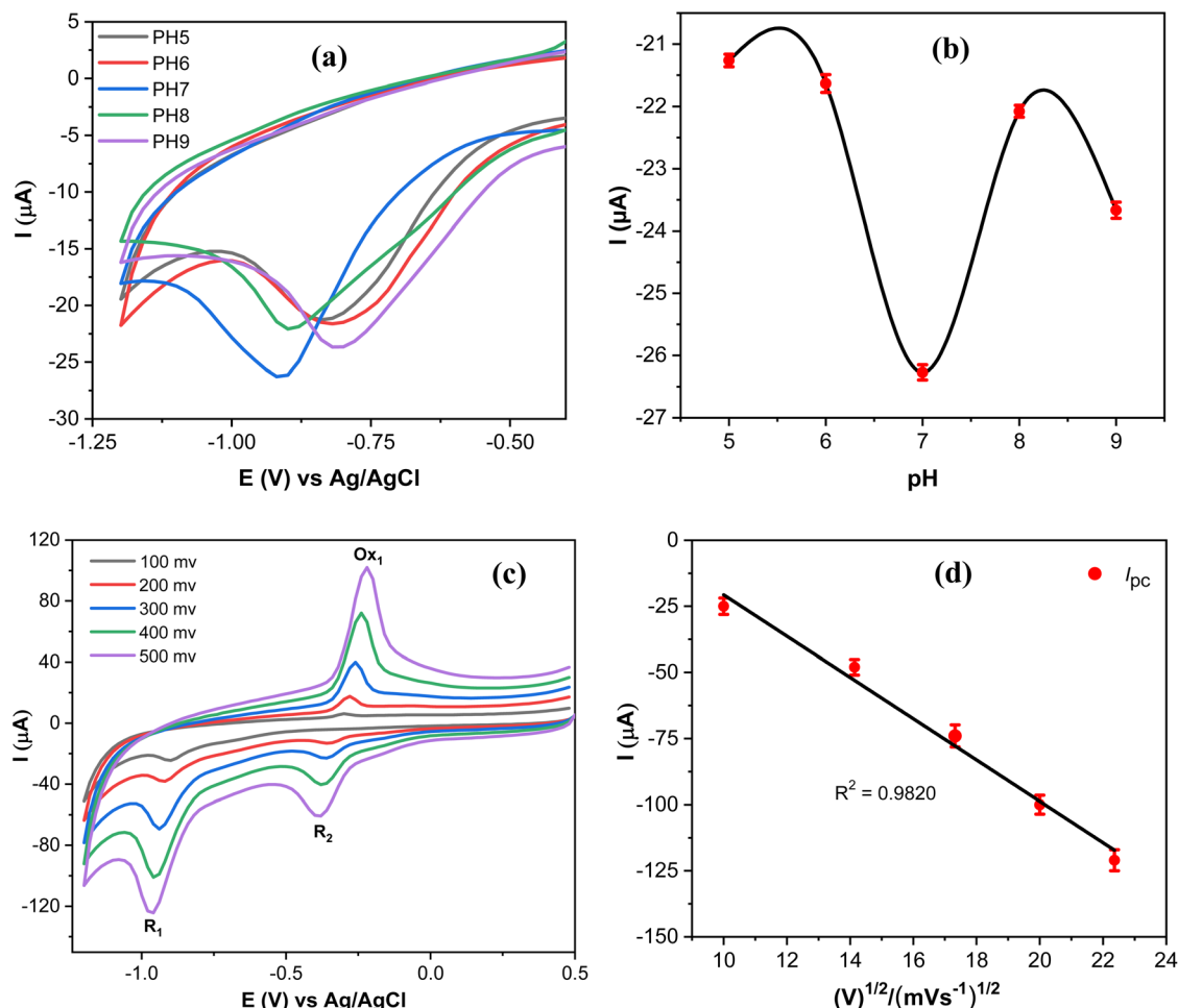
Fig. 9 (a) CV curves obtained at AgNPs@GO/IL@SPCE in 0.1 mol \text{L}^{-1} PBS containing 20 \mu\text{mol L}^{-1} MP at different pH; scan rate 100 mV \text{s}^{-1} . (b) The correlation between the pH and the reduction peak current of MP. (c) CV curves of 20 \mu\text{mol L}^{-1} PM in 0.1 mol \text{L}^{-1} PBS (pH 7) at different scan rates. (d) A graph depicting the peak currents of MP reduction ( R_1 ) plotted against the square root of the scan rate. Note: geometric area of the working electrode: 7 \text{mm}^2 .
