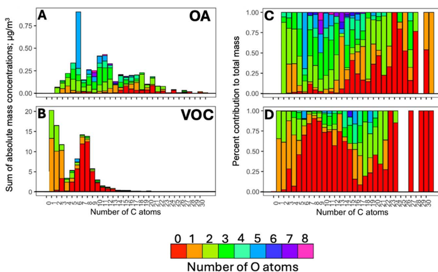
Fig. 1 Overview of the mass distribution across the different chemical compositions of compounds detected with the PTR-ToF-MS, (A) in the particle phase, and (B) in the gas phase. Corresponding percent contributions are shown in (C) and (D).
