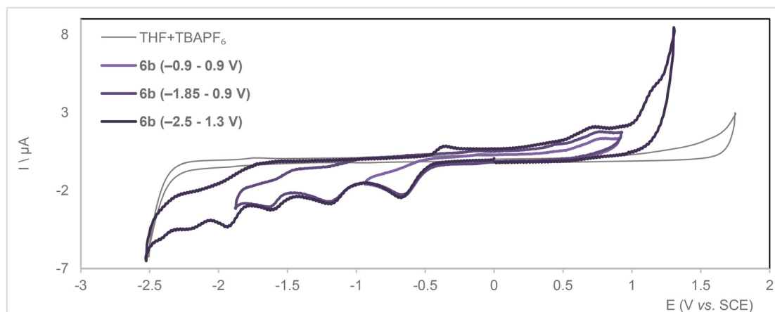
Fig. 7 Cyclic voltammograms for compound 6b (bottom) ([C] = 1 mM) recorded over different voltage ranges under Ar in dry THF with 0.1 M TBA [PF 6 ] supporting electrolyte ( \nu = 0.2 \text{ V s}^{-1} ).
