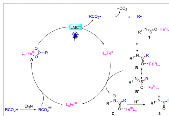
Scheme 5 Proposed mechanism.
