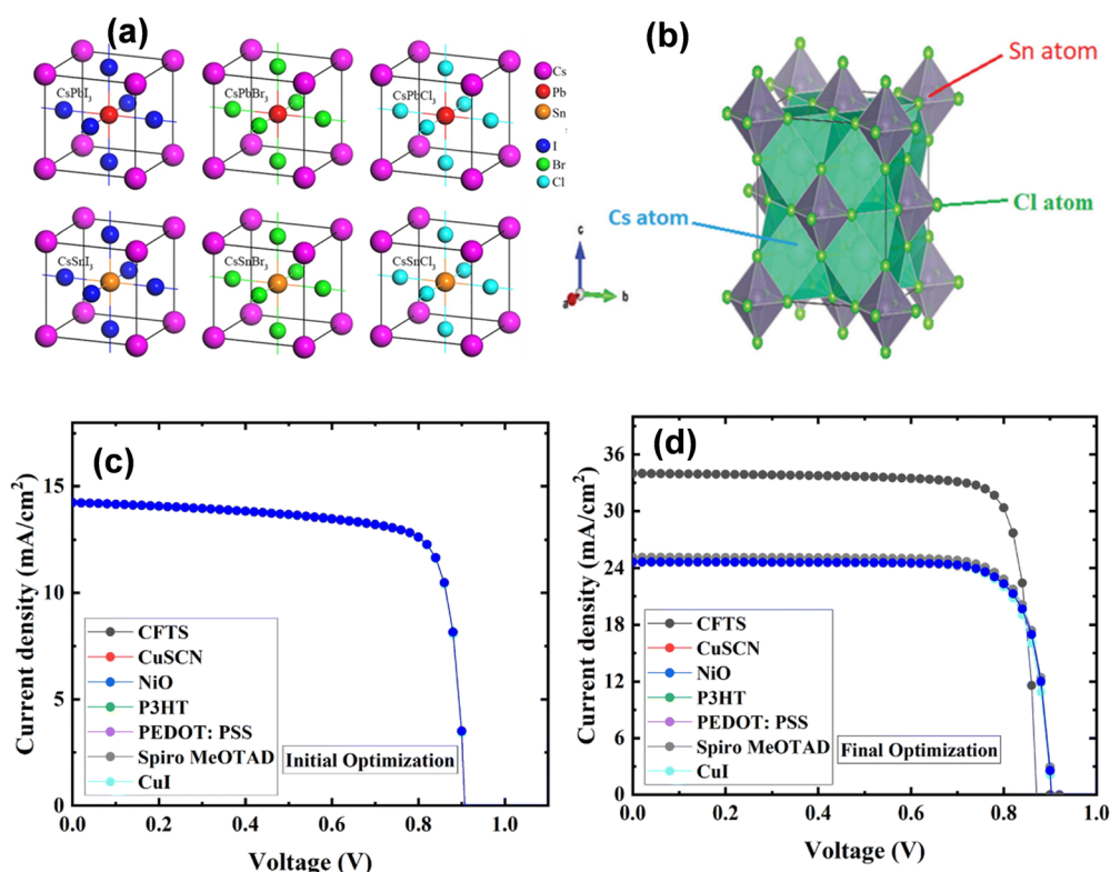
Fig. 3 Representation of unit cells of \text{CsSnX}_3 (B = Pb and Sn) composed of different halide anions. Reproduced with permission from ref. 126, copyright 2017, Nature Scientific Reports. (b) Schematic of the crystal structure of defect perovskite \text{Cs}_2\text{SnCl}_6 (green color represents Cl atoms, while Cs atoms are positioned at the interstitial spaces). Reproduced with permission from ref. 130, copyright 2019, RSC. (c) and (d) Current density–voltage curve of the initial and final optimized structure of ITO/PCBM/ \text{CsSnI}_3 /HTL/Se, respectively. Reproduced with permission from ref. 131, copyright 2023, RSC.
