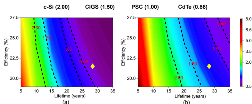
Fig. 4 The influence of PCE and lifetime on the average normalized environmental impacts of Alt-1 (a) and Alt-2 (b) ld-PSC. The diamond icon (yellow) represents the average normalized environmental impact of Alt-1 ld-PSC (i.e., 0.76) and Alt-2 ld-PSC (1.16), corresponding to the current lifetime and PCE. The average normalized environmental impact of c-Si, CdTe, and CIGS is 2.00, 0.86, and 1.50 respectively (as outlined in Table 4). Additionally, Fig. 4a and b also show the environmental impact of ld-PSC equivalent to PSC and commercial technologies in black dashed lines.
