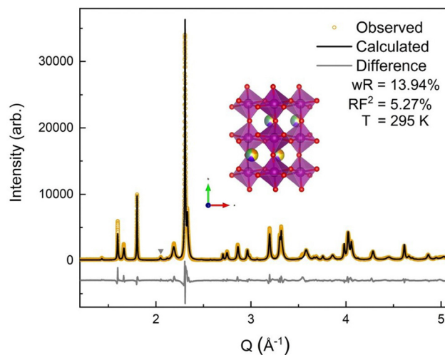
Fig. 3 SXR pattern collected at Argonne National Laboratory's 11-BM beamline with a wavelength of 0.4582 Å. The orange circles show the collected data with the black line denoting the calculated diffraction pattern fit using the GSAS-II program, a wR of 13.94% was obtained with a main phase RF^2 of 5.27%. The gray triangle denotes the impurity peak. The light gray line shows the difference curve, (data-fit) shifted down for visibility.
