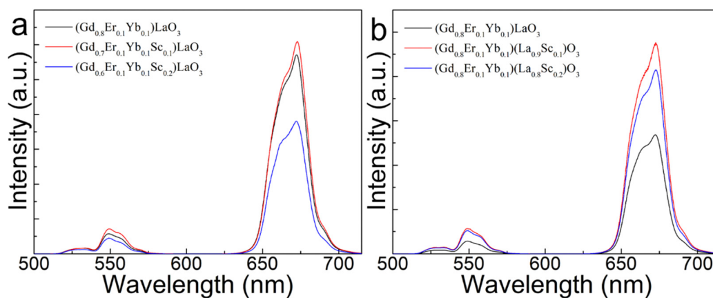
Fig. 4 UCL spectra of (\text{Gd}_{0.8-x}\text{Er}_{0.1}\text{Yb}_{0.1}\text{Sc}_x)\text{LaO}_3 ( x = 0, 0.1, 0.2 ) (a) and (\text{Gd}_{0.8}\text{Er}_{0.1}\text{Yb}_{0.1})(\text{La}_{1-x}\text{Sc}_x)\text{O}_3 ( x = 0, 0.1, 0.2 ) (b) under 980 nm laser excitation.
