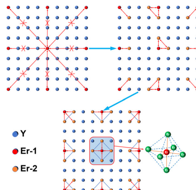
Fig. 7 Schematic diagram of \text{Er}^{3+} ion doping energy transfer.
