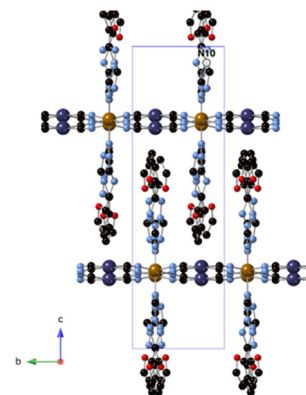
Fig. 1 ac (top) and bc (bottom) plane projections of 1 (C (black), N (blue), O (red), Fe (orange), Pt (dark blue)). Only one of the two possible configurations are shown. Hydrogen atoms have been omitted for clarity.
