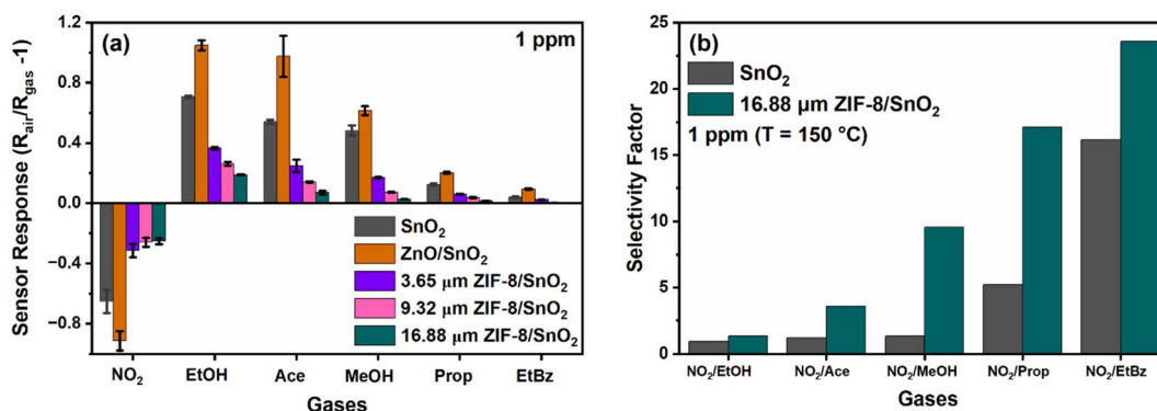
Fig. 5 (a) Responsivity bar plot of the SnO 2 , ZnO/SnO 2 and 3.65 \mu m (thin), 9.32 \mu m (medium) and 16.88 \mu m (thick) ZIF-8/SnO 2 dual layer sensors towards 1 ppm of nitrogen dioxide (NO 2 ), ethanol (EtOH), acetone (Ace), methanol (MeOH), propane (Prop) and ethyl benzene (EtBz) at 150 °C. (b) Selectivity factor bar plot representing R(\text{NO}_2)/R(\text{target gas}) calculated at 1 ppm for SnO 2 and 16.88 \mu m (thick) ZIF-8/SnO 2 hierarchical dual layer sensors gas sensor at 150 °C toward nitrogen dioxide (NO 2 ), ethanol (EtOH), acetone (Ace), methanol (MeOH), propane (Prop) and ethyl benzene (EtBz) at 150 °C.
