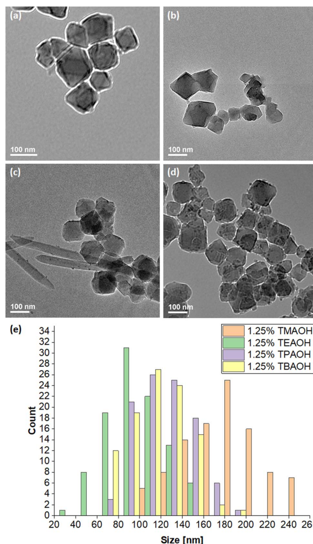
Fig. 6 TEM images of MIL-101(Cr) prepared from 1.25% quaternary alkylammonium hydroxide solutions from (a) TMAOH, (b) TEAOH, (c) TPAOH and (d) TBAOH with scale bars at 100 nm. (e) The particle size distribution of MIL-101(Cr) synthesised using the above quaternary alkylammonium hydroxide solutions.
