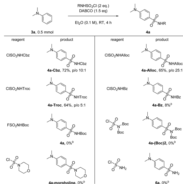
Scheme 5 Reaction of 3a with other N -sulfonamide precursors. Cbz = CO 2 CH 2 Ph, Alloc = CO 2 CH 2 CH=CH 2 , Troc = CO 2 CH 2 CCl 3 , and Bz = C(=O)Ph. [b] 0.1 mmol scale.
