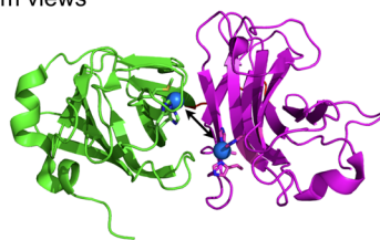
Fig. 2 Uncoupled binuclear copper-containing monooxygenases, PHM and D \beta H. (a) and (b) reactions catalyzed by PHM and D \beta H, respectively; (c) X-ray structure of PHM from Rattus norvegicus showing the two domains (Cu M domain in green and Cu H domain in magenta) connected by a loop (in blue) in which each domain binds a single copper atom spaced from each other by approximately 11 Å and (d) structure of the Cu M -superoxido intermediate in PHM (PDB ID 1opm); (e) and (f) X-ray structure of the human D \beta H (PDB ID 4zel) showing the open (e) and the closed (f) forms. Only the Cu M domain of the closed form contains a copper atom, the other copper ions (red sphere) are manually placed.
