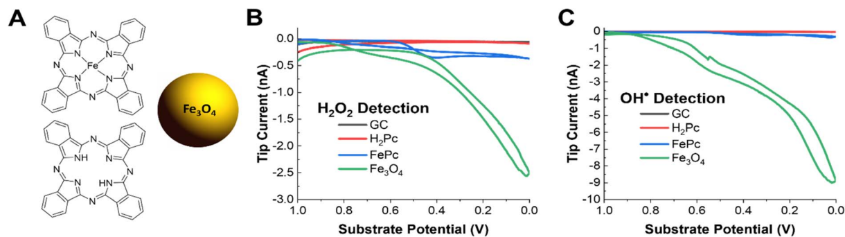
Fig. 4 SECM measurements of \text{OH}^\bullet and \text{H}_2\text{O}_2 generation on active site model systems. (A) The structure of iron(II) phthalocyanine, phthalocyanine, and schematic of the 20 nm \text{Fe}_3\text{O}_4 nanoparticle. (B) \text{H}_2\text{O}_2 SG/TC response of each model catalyst system on a GC electrode in oxygen-saturated 0.5 M \text{H}_2\text{SO}_4 . (C) \text{OH}^\bullet SG/TC detection using 50 mM DMPO of each model catalyst system on a GC electrode in oxygen saturated 0.5 M \text{H}_2\text{SO}_4 .
