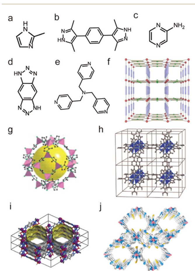
Fig. 9 The structures of representative Co(II)-MOFs and the used ligands. (a) The MeIM ligand. (b) The H 2 bdpb ligand. (c) The pyz-NH 2 ligand. (d) The H 2 bbta ligand. (e) The TPMA ligand. (f) ZJU-75. Reproduced from ref. 124 with permission from Wiley, Copyright 2023. (g) ZIF-67. Reproduced from ref. 120 with permission from The American Association for the Advancement of Science, Copyright 2008. (h) MFU-1. Reproduced from ref. 121 with permission from Wiley, Copyright 2009. (i) MAF-X27-Cl. Reproduced from ref. 122 with permission from the American Chemical Society, Copyright 2016. (j) FJIH-30. Reproduced from ref. 123 with permission from the American Chemical Society, Copyright 2020.
