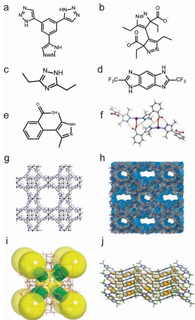
Fig. 11 The structures of representative Cu/Ag-MOFs and the used ligands. (a) The H_3BTri ligand. (b) The TBPZ ligand (TBPZ = 3,3',5,5'-tetraethyl-4,4'-bipyrazolate). (c) The Hetz ligand. (d) The H_2fbdim ligand. (e) The o-H_2mpba ligand. (f) [Ag_2(o-Hmpba)_2(o-H_2mpba)_2] . Reproduced from ref. 135 with permission from Wiley, Copyright 2020. (g) Cu-BTTri. Reproduced from ref. 130 with permission from the American Chemical Society, Copyright 2009. (h) Cu_2TBPZ . Reproduced from ref. 133 with permission from Wiley, Copyright 2014. (i) MAF-2. Reproduced from ref. 131 with permission from the American Chemical Society, Copyright 2008. (j) MAF-41. Reproduced from ref. 132 with permission from Springer Nature, Copyright 2019.
