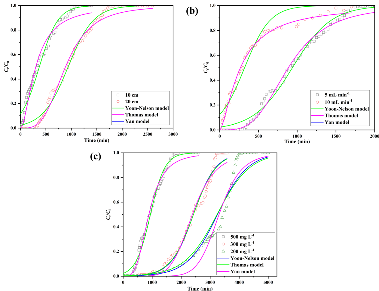
Fig. 16 Effect of (a) packed-bed height (Z: 10–20 cm; Q : 5 mL min -1 ; C_0 : 500 mg L -1 ), (b) inlet flow rate ( Q : 5–10 mL min -1 ; Z: 20 cm; C_0 : 500 mg L -1 ), and (c) inlet Pb^{2+} ion concentration ( C_0 : 200, 300, and 500 mg L -1 ; Q : 5 mL min -1 ; Z: 20 cm).
