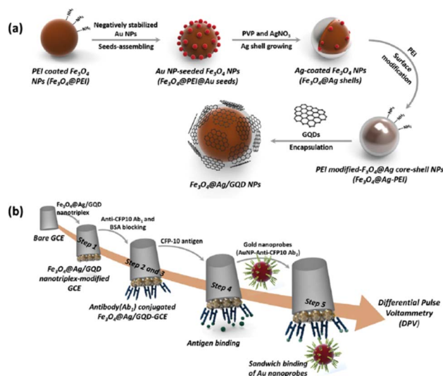
Fig. 14 Synthesis of \text{Fe}_3\text{O}_4@\text{Ag}/\text{GQD} NP nanotriplex probe (a) immunosensor preparation (b): drop casting onto the GCE (step 1), incubation with CAB (step 2), blocking with BSA (step 3), incubation with the target antigen (step 4), and incubation with the AbD-AuNPs (step 5). Reprinted with permission from ref. 232. Copyright © 2018 Elsevier Ltd.
