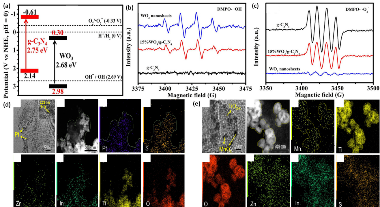
Fig. 19 (a) Band arrangements of g-C 3 N 4 and WO 3 nanosheets. EPR spectra showing (b) DMPO·OH in an aqueous solution and (c) DMPO·O 2 ·- in a methanol dispersion, with g-C 3 N 4 , WO 3 nanosheets, and 15%WO 3 /g-C 3 N 4 photocatalysts. The figures are adapted with permission from ref. 100. Copyright 2019, Elsevier. (d) TEM, STEM, and EDX spectroscopy element mapping images of the Pt photodeposited O-ZIS/TiO 2-x heterojunction. (e) TEM, STEM, and EDX element mapping images of the MnO x photodeposited O-ZIS/TiO 2-x photocatalyst. The figures are adapted with permission from ref. 175. Copyright 2022, Elsevier.
