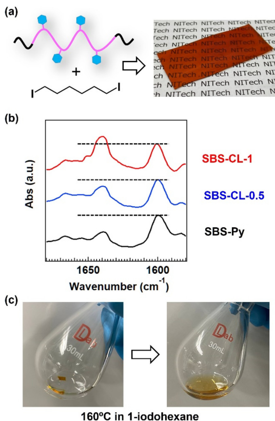
Fig. 3 (a) Macroscopic appearance of the cross-linked sample, SBS-CL-1. (b) FT-IR spectra of SBS-Py, SBS-CL-0.5, and SBS-CL-1, focusing on the peaks from free and quaternized pyridines. The dotted line is a guide to the eye to see the change in relative intensity between the peaks at 1600 \text{ cm}^{-1} and 1640 \text{ cm}^{-1} . (c) De-crosslinking behavior of SBS-CL-1 in 1-iodohexane.
