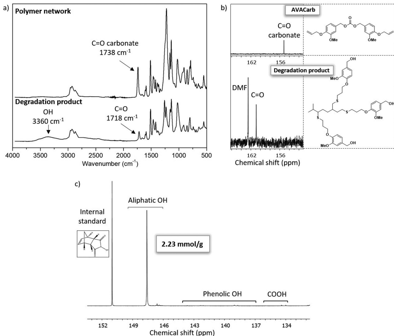
Fig. 8 (a) FTIR spectra of the polymer network (top) and degradation product (bottom), (b) zoom on the 13 C NMR spectra of the AVACarb (top) and degradation product (bottom), (c) 31 P NMR spectrum of the phosphorylated degradation product.
