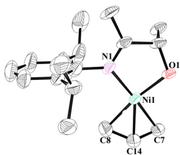
Fig. 1 The molecular structure of Ni1 (CCDC229534†). Hydrogen atoms were omitted for clarity, and ellipsoids were set at 30% probability. Selected bond lengths (Å) and angles (°): Ni1–O1 1.893 (4), Ni1–N1 1.897 (5), Ni1–C7 2.007 (7), Ni1–C8 1.989 (8), Ni1–C14 1.998 (13); N1–Ni1–O1 85.2 (2), O1–Ni1–C7 99.5 (3), N1–Ni1–C8 101.2 (3), N1–Ni1–C14 101.2 (3), C7–Ni1–C8 74.2 (3).
