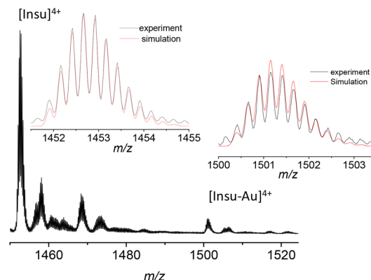
Fig. 1 Zoom of the variable temperature-nano electrospray ionization (VT-nano-ESI) MS spectrum of insulin–gold conjugate, corresponding to the 4+ charge state (Insu for Insulin). Insets. Isotopic pattern (black: experimental, and red: simulation) of insulin (C 257 H 383 N 65 O 77 S 6 ) on the left and of insulin with Au(III) (C 257 H 380 N 65 O 77 S 6 Au) on the right. The other minor peaks are mostly alkali adducts.
