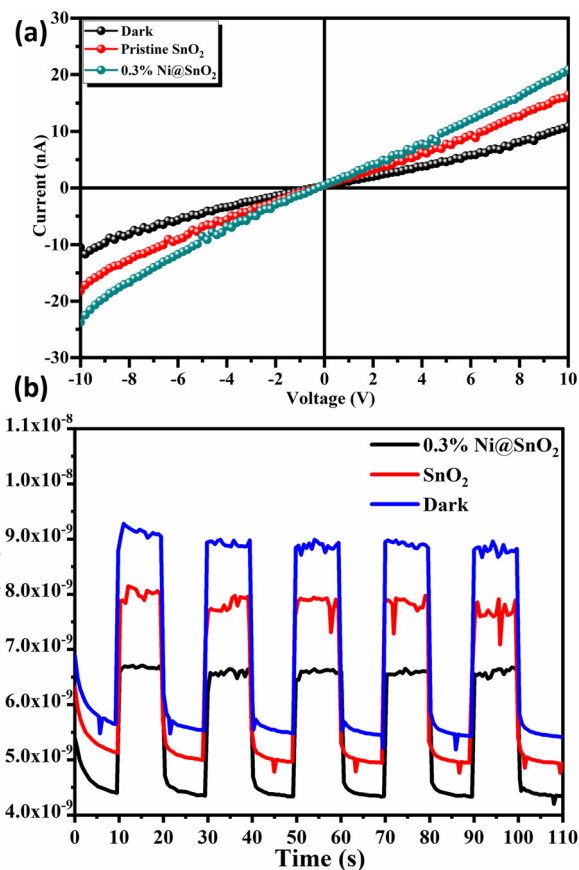
Fig. 13 (a) I - V characteristics and (b) photo-response of pristine \text{SnO}_2 and 0.3% \text{Ni@SnO}_2 photodetectors.
