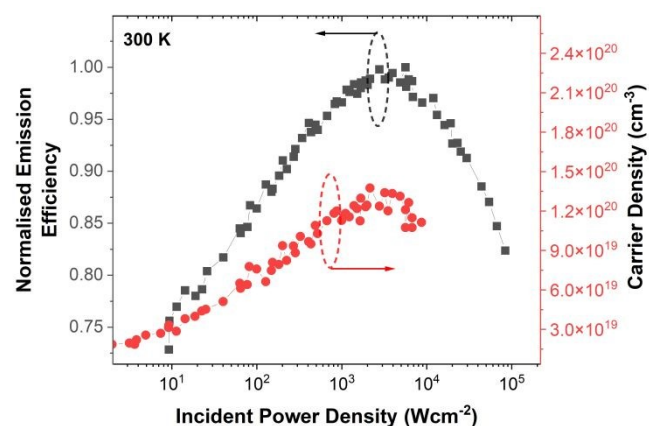
Figure 5. Emission efficiency and carrier density determined by PL and PR measurements, respectively, for the 5 nm zb-MQW sample as a function of resonant steady-state laser excitation power density at 300 K.
