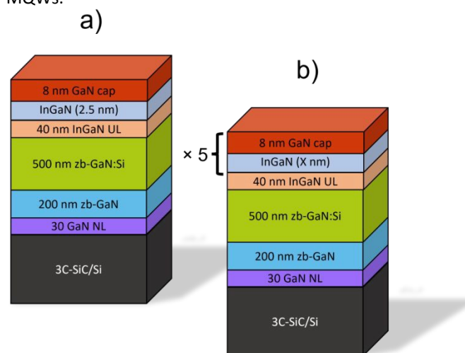
Figure 1. Diagram of a) zb-SQW and b) MQW samples used in this study.
