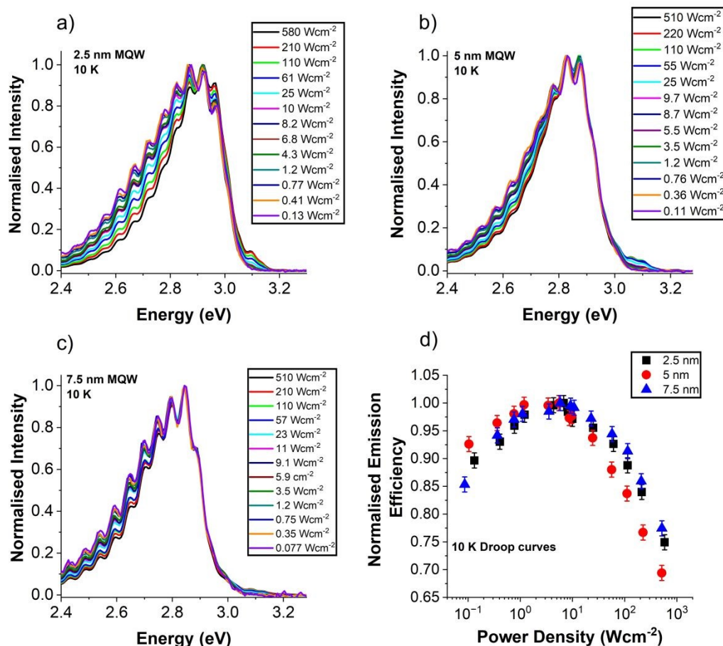
Figure 3. Power density dependent emission spectrum for MQWs with well widths of a) 2.5 nm, b) 5 nm, and c) 7.5 nm. d) 10 K droop response comparison of the MQW samples.
