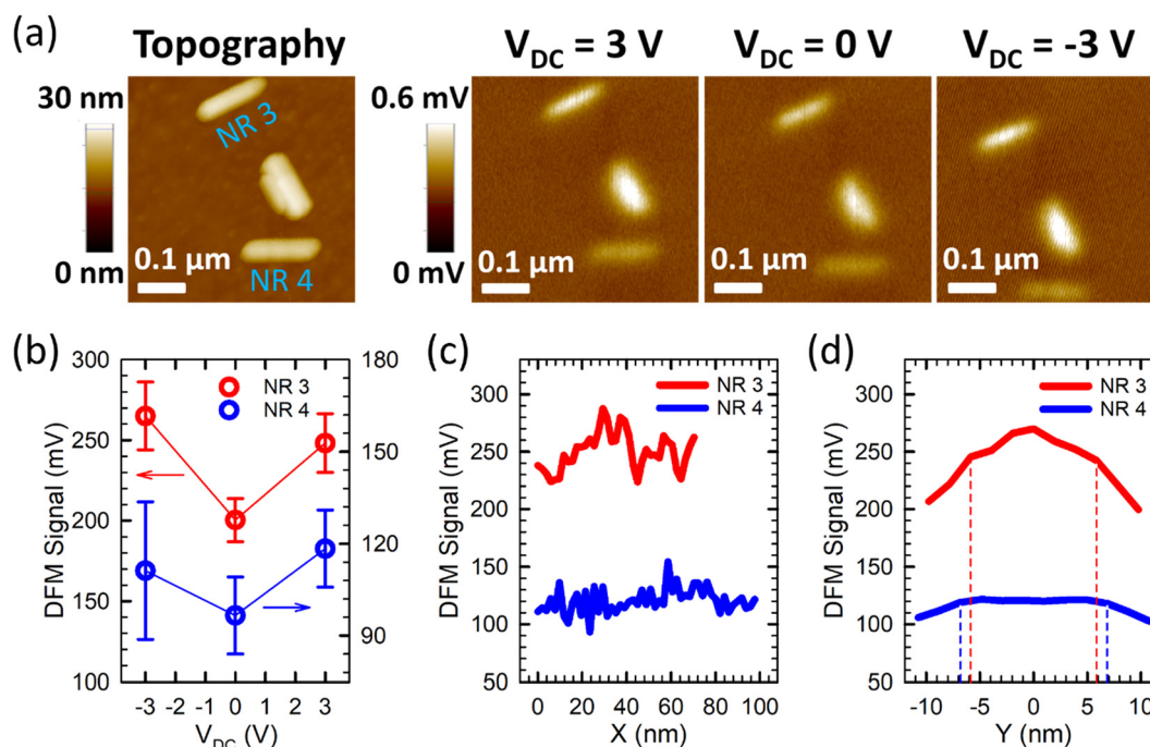
Fig. 3 (a) Topographical image and dielectric response images of an area with two well-separated \text{CsPbBr}_3 nanorods, NR 3 (diameter 12 \pm 1 nm) and NR 4 (diameter 10 \pm 1 nm), 56 days after the sample was synthesized. (b) DFM signal as a function of V_{\text{DC}} for NR 3 and NR 4. (c) DFM signal as a function of X extracted from the dielectric response images for NR 3 and NR 4 at V_{\text{DC}} = 3 V. (d) DFM signal as a function of Y extracted from the dielectric response images for NR 3 and NR 4 at V_{\text{DC}} = 3 V, where the boundaries of the Y -range with nearly constant DFM signals (or the Y -range in which the DFM signals changed slower) are indicated by dashed lines.
