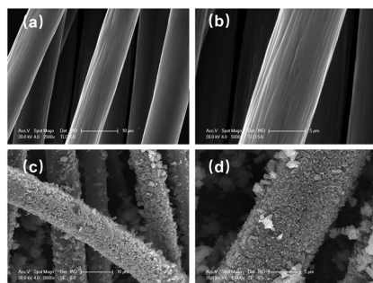
Fig. 4 SEM images of (a and b) H 2 O 2 -pretreated CC substrate and (c and d) CoNi 0.5 -MOF/CC at different magnifications.
