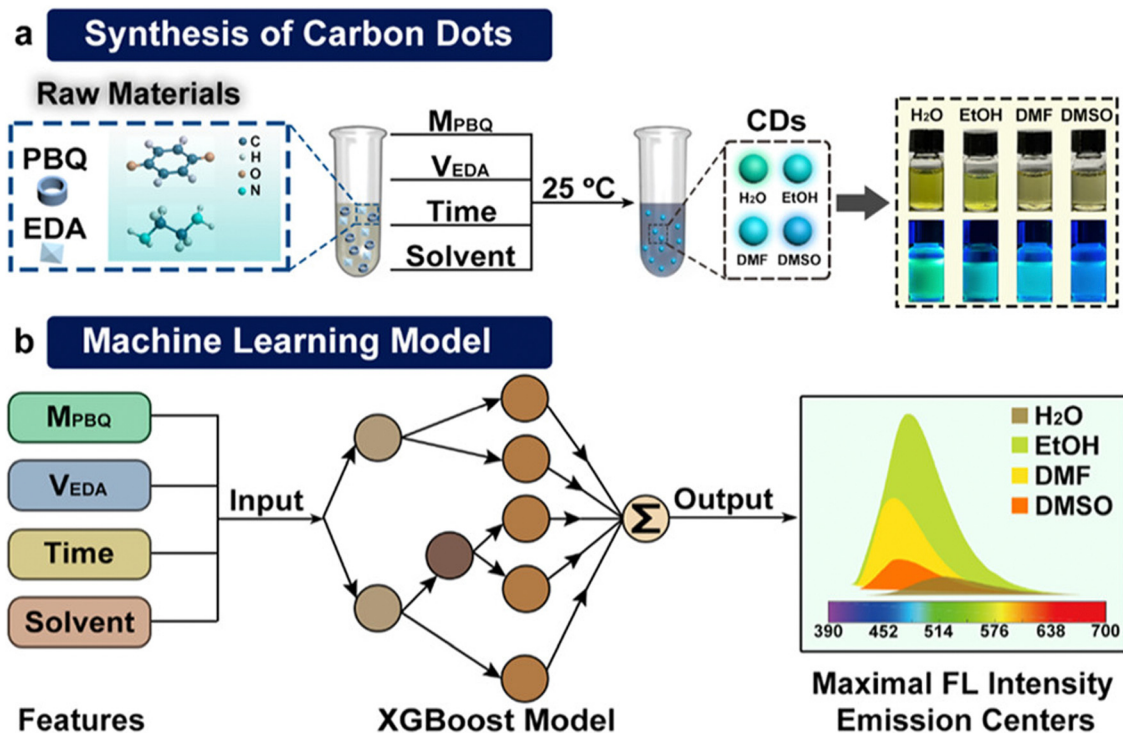
Fig. 4 Schematic illustration of machine learning guiding the synthesis of CDs. (a) Synthetic process of CDs. (b) Prediction of CD optical properties using machine learning models. Reprinted with permission from ref. 119. Copyright 2022 American Chemical Society.
