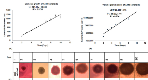
Fig. 6 Diameter (A) and volume (B) growth curve of A549 spheroid cells in 10 days, which shows VDT = 23.44 \pm 1.4 h, mean \pm SD ( n = 3 ). Also, the shape of the spheroid has been shown in 200 \mu\text{m} resolution (Olympus microscope, USA) (C).
