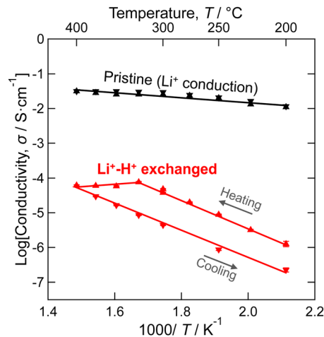
Fig. 5 Arrhenius-type plot of total electrical conductivity of the 91% Li^+H^+ exchanged LLZ dense bodies measured in heating and subsequent cooling process. Conductivity of the pristine LLZ is also shown for comparison.
