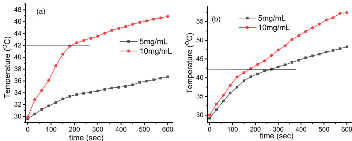
Fig. 7 Induction heating (temperature vs. time) profile of the Fe 3 O 4 @SiO 2 @GdPO 4 :Tb 3+ ,Ce 3+ nanocomposites at different concentrations and magnetic field strengths (Hf) (a) 3.05 \times 10^6 (kA m -1 s -1 ) and (b) 4.58 \times 10^6 (kA m -1 s -1 ) maintained at a fixed applied frequency of 178 kHz.
