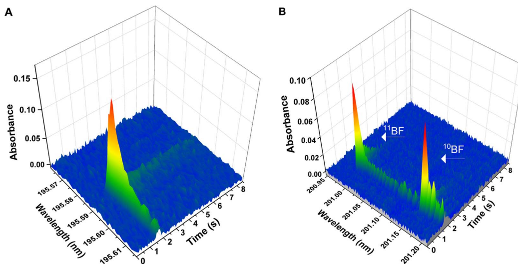
Fig. 1 Wavelength- and time-resolved spectra for the two different BF transitions deployed in the work. Spectra were obtained with aqueous standard solutions and deploying the temperature program presented on Table 1 (chemical modifiers: citric acid 150 \mu\text{g} , Ca 10 \mu\text{g} , W_{\text{permanent}} 250 \mu\text{g} ). (A) Spectrum for the X^1\Sigma \rightarrow A^1\Pi (0,0) transition generated using 10 ng of B elemental standard of natural isotopic composition. The central pixel was adjusted at 195.589 nm (detection pixel). (B) Spectrum for the X^1\Sigma - A^1\Pi (1,0) transition, showing two separated peaks for ^{10}\text{BF} and ^{11}\text{BF} . Spectrum generated using two isotopic B standards (approximately 50 ng of each boron isotope). The central pixel was set at 201.08 nm; ^{11}\text{BF} maximum peak is found at 200.993 nm, and ^{10}\text{BF} maximum at 201.160 nm.
