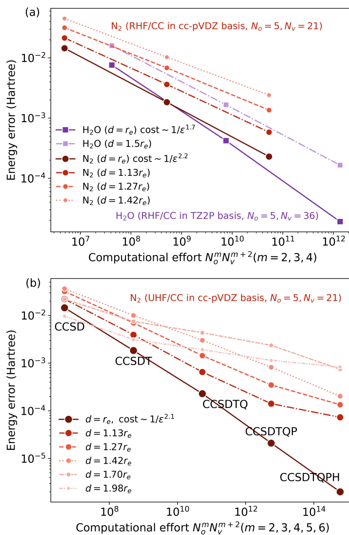
Fig. 2 Energy error of nitrogen and water molecules at equilibrium r_e and stretched (multiples of r_e ) bond lengths, as a function of the level of coupled cluster truncation, against a computational cost metric. (a) and (b) show the data computed using RHF/CC and UHF/CC, respectively. Data taken from Refs. 35 and 59 .
