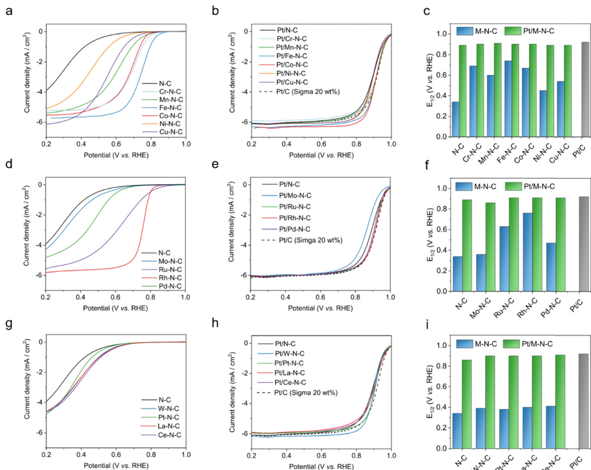
Fig. 4 ORR performance evaluated by RDE in 0.1 M HClO 4 with a scan speed of 5 mV s -1 . (a)–(c) Half-wave potentials for bare M–N–C catalysts, Pt supported M–N–C (Pt/M–N–C) and summary of half-wave potentials for 3d metals. (d)–(f) Half-wave potential for 4d metals. (g)–(i) Half-wave potentials for 5d and f metals.
