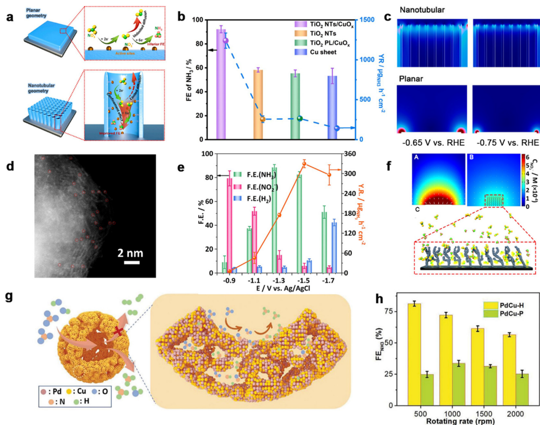
Fig. 8 Confinement effect. (a) Schematic illustration of NO 3 - -to-NH 3 reduction over an electrode with nanotubular geometries. (b) Comparison of FE of NH 3 over TiO 2 NTs/CuO x , TiO 2 NTs, TiO 2 PL/CuO x and Cu sheet at -0.75 V vs. RHE. (c) Simulated NO 2 - concentration distribution on nanotubular and planar electrodes. 138 Copyright 2022, Elsevier. (d) Aberration-corrected HAADF-STEM image of Cu SAAs. (e) Faradaic efficiency of products and NH 3 yield rate of Cu SAAs, Cu foil, and PPy-C at -0.9 V (vs. RHE). (f) A flat electrode (A) and a porous electrode (B) at the same potential, where NO 3 - /NO 2 - and NO 2 - /NH 4 + transformation simultaneously occur. Schematic diffusion process of NO 2 - in interconnecting networks (C). 139 Copyright 2023. (f) Schematic illustrations for NitRR over PdCu-P with high selectivity. (g) The relationships between FE of NH 3 and rotating rates over PdCu-H, PdCu-P, and Pd-P. 140 Copyright 2023, Wiley.
