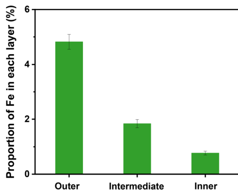
Fig. 2 XRF analysis of Fe content in the three layers (outer layer, intermediate layer, and inner layer) of the used PCF.
