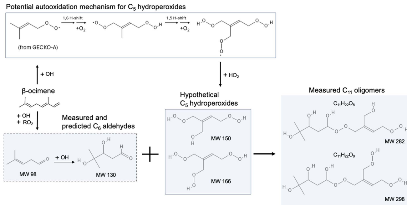
Fig. 5 One possible reaction mechanism that could generate C 11 oligomers from \beta -ocimene oxidation. The C 6 aldehydes in the shaded box with a dashed outline are predicted by GECKO-A modeling and have matching neutral masses in the ESI HRMS spectrum.
