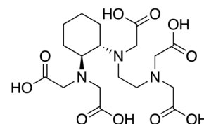
CHX-A''-DTPA
