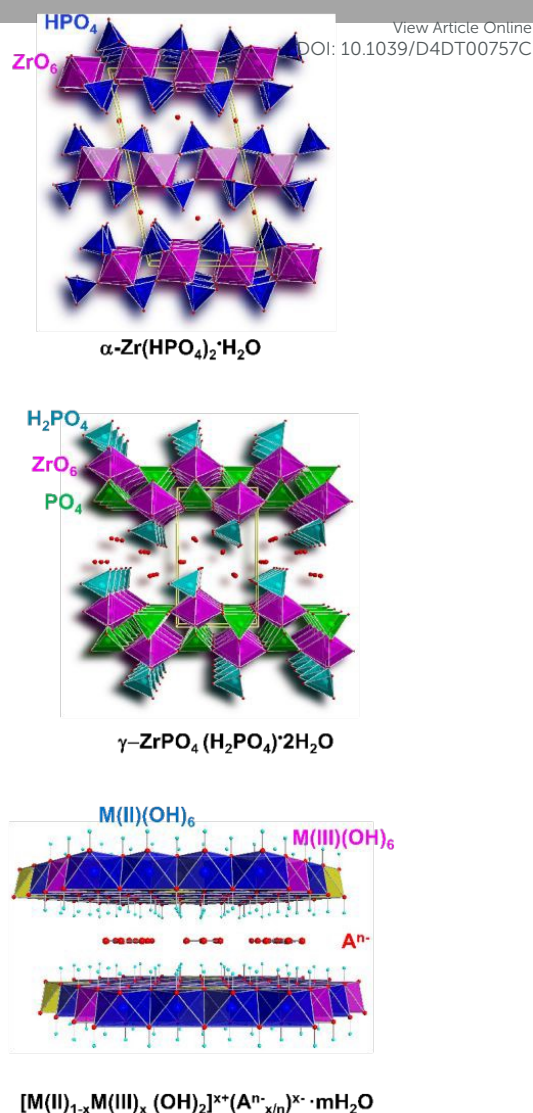
Fig. 2 Schematic view of \alpha -ZrP, \gamma -ZrP and LDHs structures.
