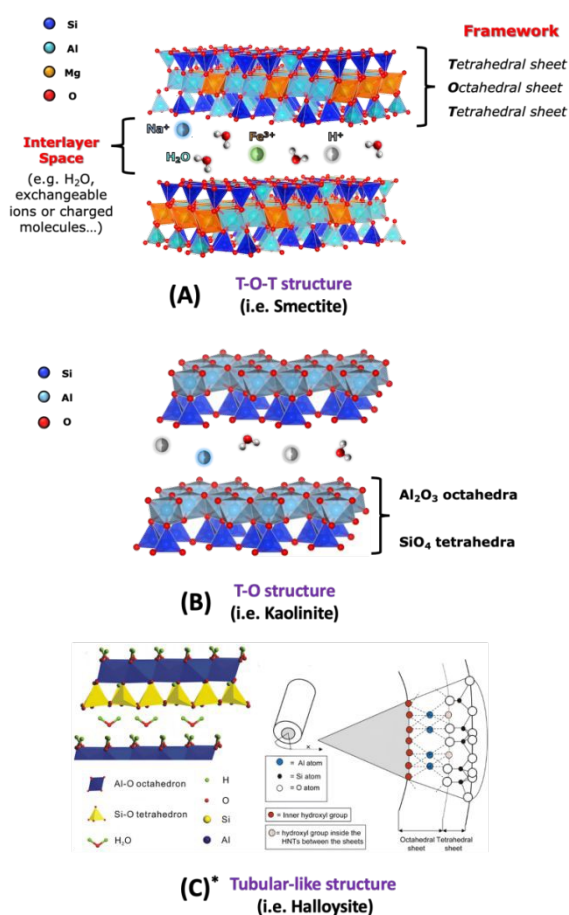
Fig. 1 Schematic view of different clay structures: T-O-T (A), T-O (B) structures and tubular-like structure (C* is adapted with permission from Ref. 1., Copyright 2020 MDPI).
