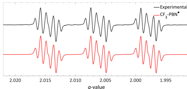
Fig. 17 Room temperature EPR spectrum of the \text{CF}_3 -PBN ^\bullet adduct ( g_{\text{iso}} = 2.0061 , {}^{19}\text{F} a_{\text{iso}} = 0.15 mT, {}^{14}\text{N} a_{\text{iso}} = 1.42 mT and {}^1\text{H} a_{\text{iso}} = 0.22 mT) after generation due to reduction of the sulfonium salt by NMM in acetonitrile. Further experimental and simulation details are reported in the ESI.†
