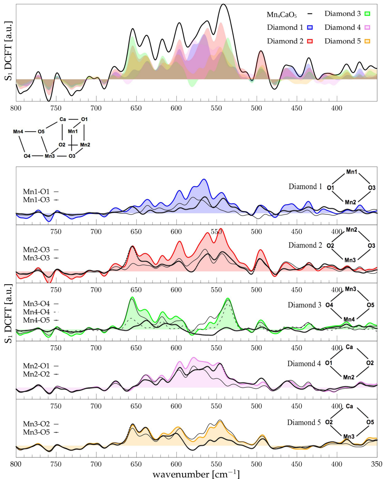
Fig. 4 The top panel displays the FT of the dipole correlation for the Mn_4Ca cluster (black line) and the diamond subunits (colored areas) in the S_1 state. In the lower panels, the FT of the dipole correlation for each Mn–O moiety is compared with the same analysis for the diamond in which it is contained.
