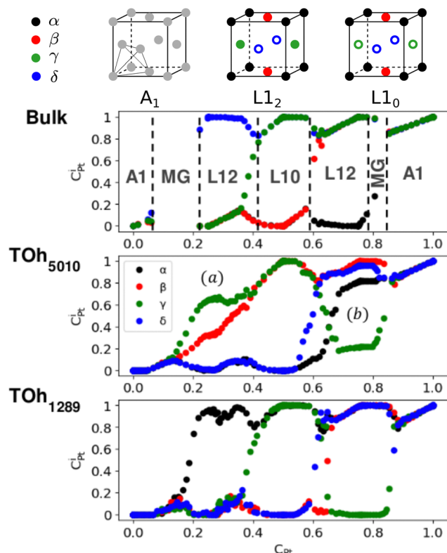
Fig. 6 Pt occupation on the different fcc sublattice sites ( C_i^{\text{Pt}} , with i = \alpha (black), \beta (red), \gamma (green) and \delta (blue)) as a function of the average composition, in the core of TOh 1289 and TOh 5010 , and as compared to the bulk case, at 300 K. Vertical dashed lines correspond to the limits of the ordered phase domain (Ni 3 Pt, NiPt and NiPt 3 ) and of the miscibility gaps in the bulk alloy. On top, the different sublattice chemical occupations of the fcc structure are schematically represented for the various relevant ordered ( L_{12} , L_{10} ) and disordered phases (grey circles), with full circles when sites are occupied by one species and empty circles when sites are occupied by the other.
