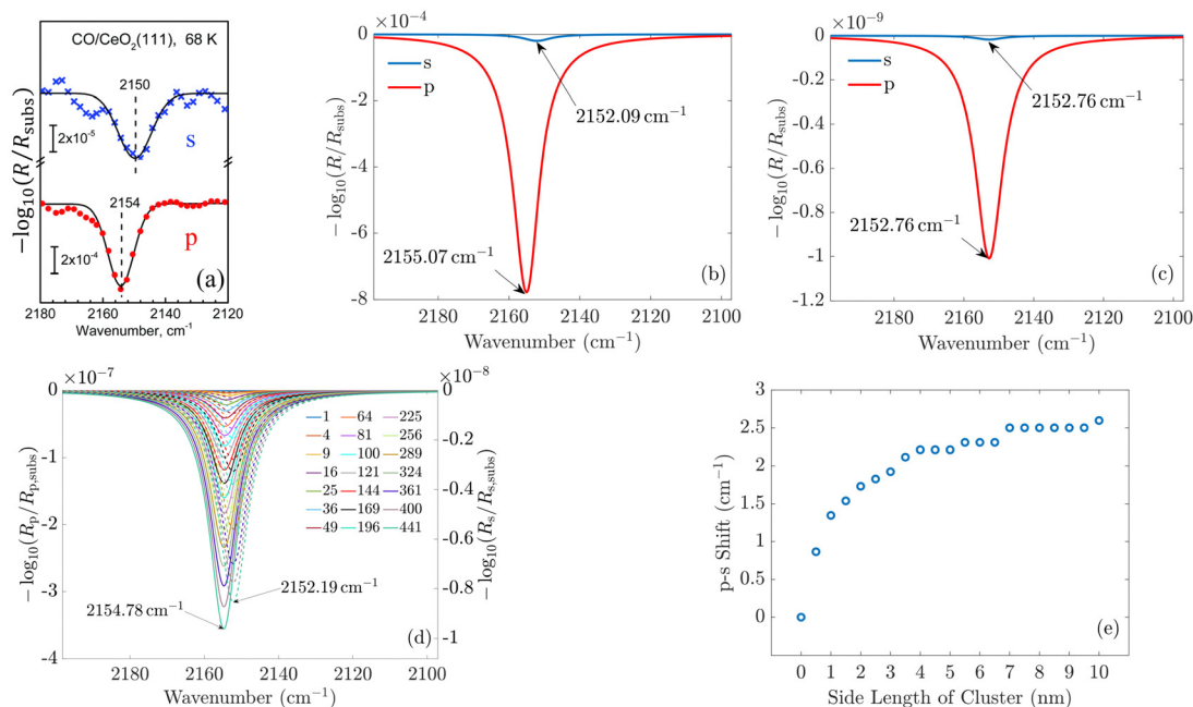
Fig. 4 (a) Experimentally measured IRRAS data and (b) simulated spectra of CO molecules on a ceria substrate. The agreement between the measured and the simulated spectra is good. The less-intense bands observed in the measurement originate from minority CO species adsorbed at defective regions of the surface (oxygen vacancies, step edges). (c) and (d) Show the simulated spectra of a single molecule on the substrate and for increasing island size, respectively. One observes that the shift between the p - and s -spectra shown in (e) increases from zero for one molecule to 2.6 \text{ cm}^{-1} . In (d), the p -spectra are solid lines, and the s -spectra are dashed lines. Fig. 4(a) is adapted with permission from ref. 15 under a CC BY-NC 3.0 Deed license. Copyright 2020, The Royal Society of Chemistry.
