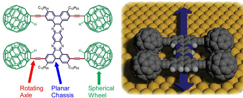
Fig. 14 A nanocar with spherical fullerene wheels, freely rotating alkyne axes, and a molecular chassis. Reprinted with permission from ref. 84. Copyright 2006 American Chemical Society.
