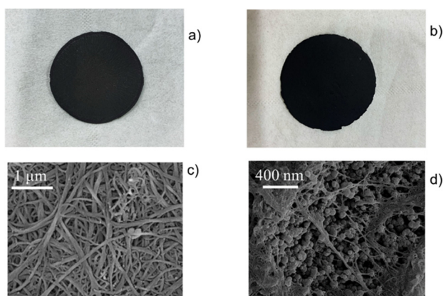
Fig. 13 Photographs of neat SWCNT-BP (a) and bioMOF@SWCNT-BP (b) obtained by integrating Cu 6 SrThreo and SWCNT-BP. (c) and (d) circular membranes own an average diameter of 41 \pm 1 mm. SEM images of SWCNT-BP (c) and bioMOF@SWCNT-BP (d). This figure is reproduced with permission from ref. 78, copyright ACS 2022.
