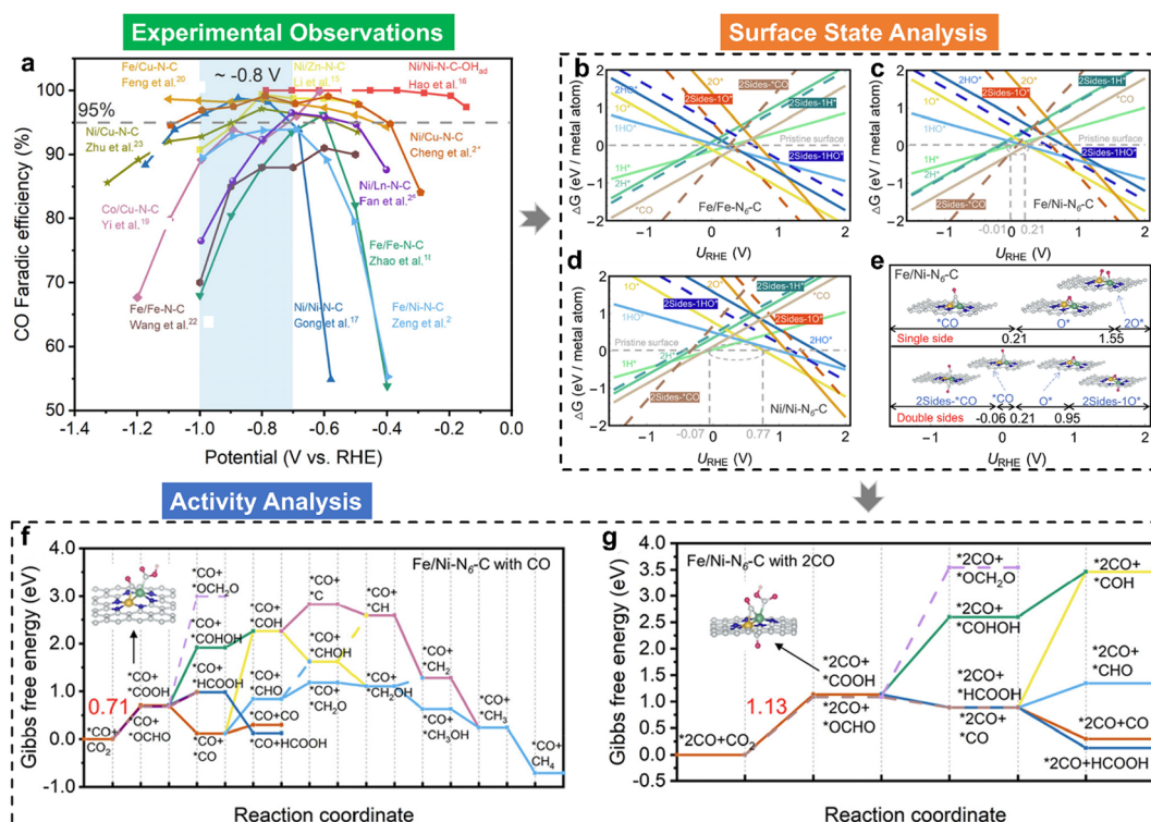
Fig. 6 (a) Comparison of the faradaic efficiency of CO (FE CO ) for various experimentally-reported dual-atom catalysts, where the FE CO data as a function of U_{RHE} were obtained from their corresponding literatures; calculated 1D surface Pourbaix diagrams of (b) Fe/Fe–N 6 –C, (c) Fe/Ni–N 6 –C, and (d) Ni/Ni–N 6 –C dual-atom catalysts, respectively, where the solid and dashed lines represent single- and double-side adsorption; (e) the surface states of Fe/Ni–N 6 –C at various potential windows, where inserts indicate the atomic configurations; Gibbs free-energy evolutions of the CO 2 RR over Fe/Ni–N 6 –C with pre-covered *CO at (f) single- and (g) double-sides, respectively. 48
